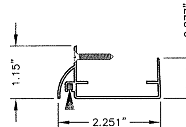
44 SWEEP
