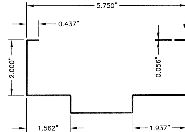
25 FRAME
