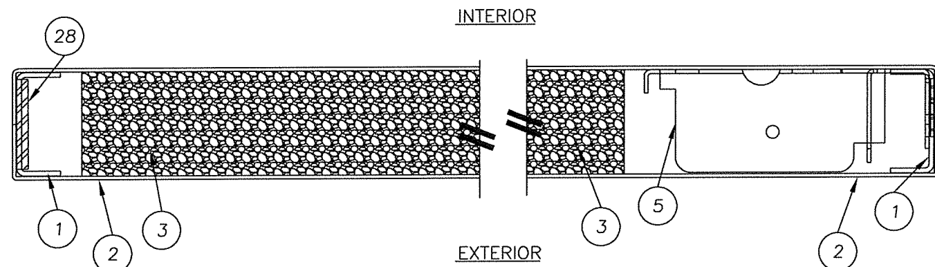
2 HORIZONTAL CROSS SECTION 2
