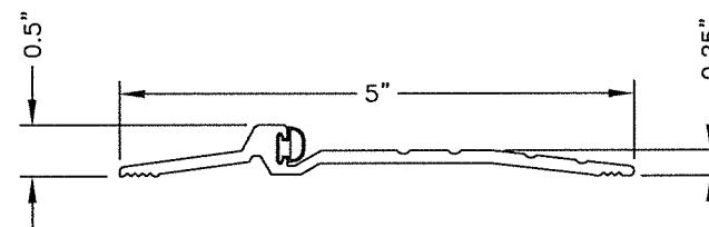
42 THRESHOLD
